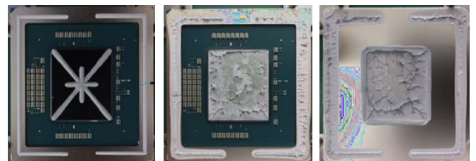
Figure 8: Typical TIM and adhesive dispense pattern
