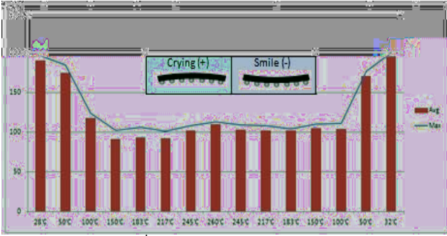
Figure 10: 3 rd DOE build package warpage data
