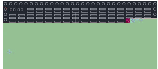
Figure 7: Typical picture of land side passives pad in large flip chip package
